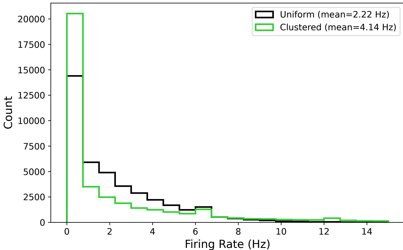
Firing Rate Distribution (Excitatory Neurons) 2 realizations \times 5 trials
