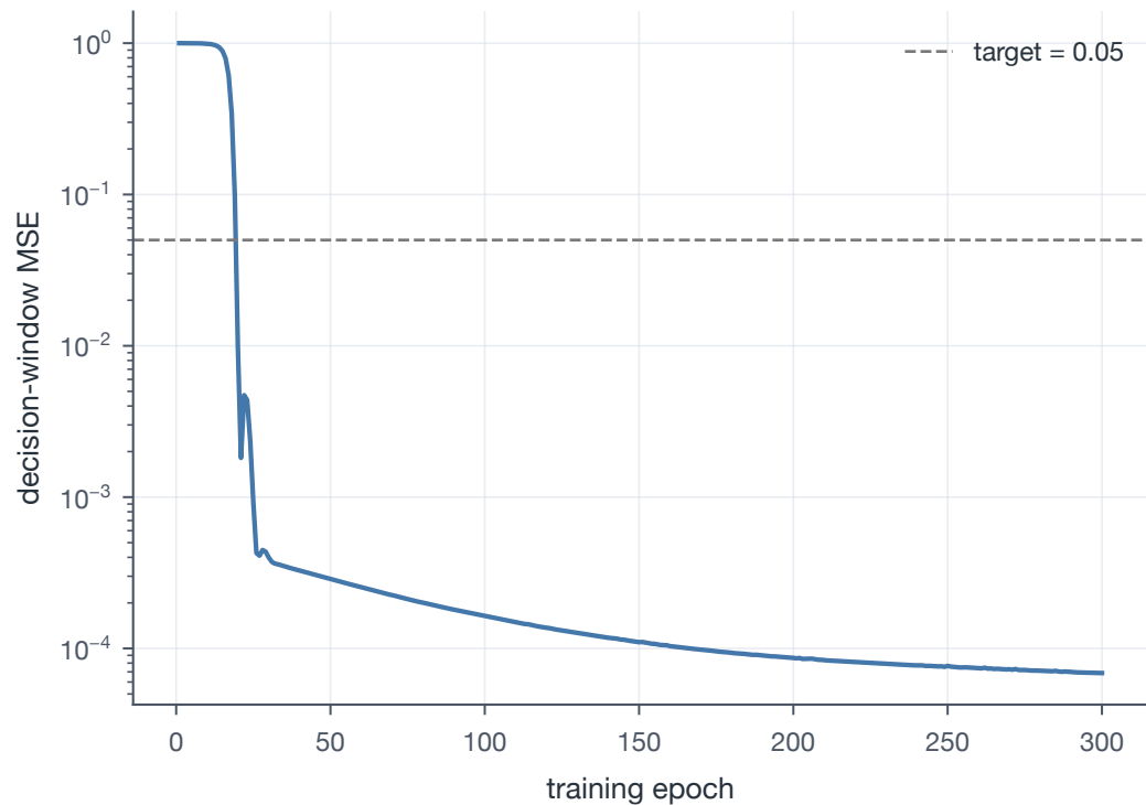
Rank-one optimization
