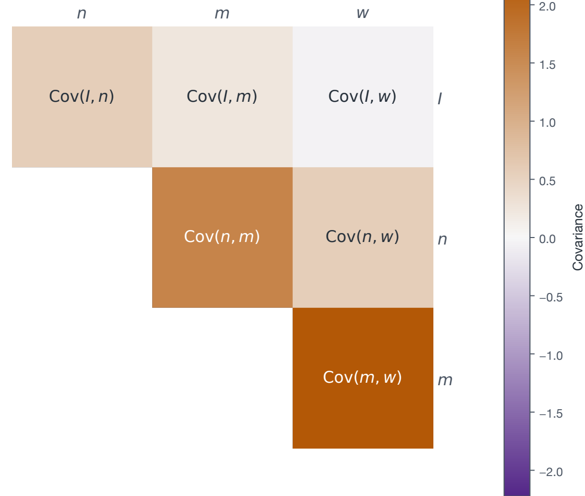
Rank-one loading covariance
