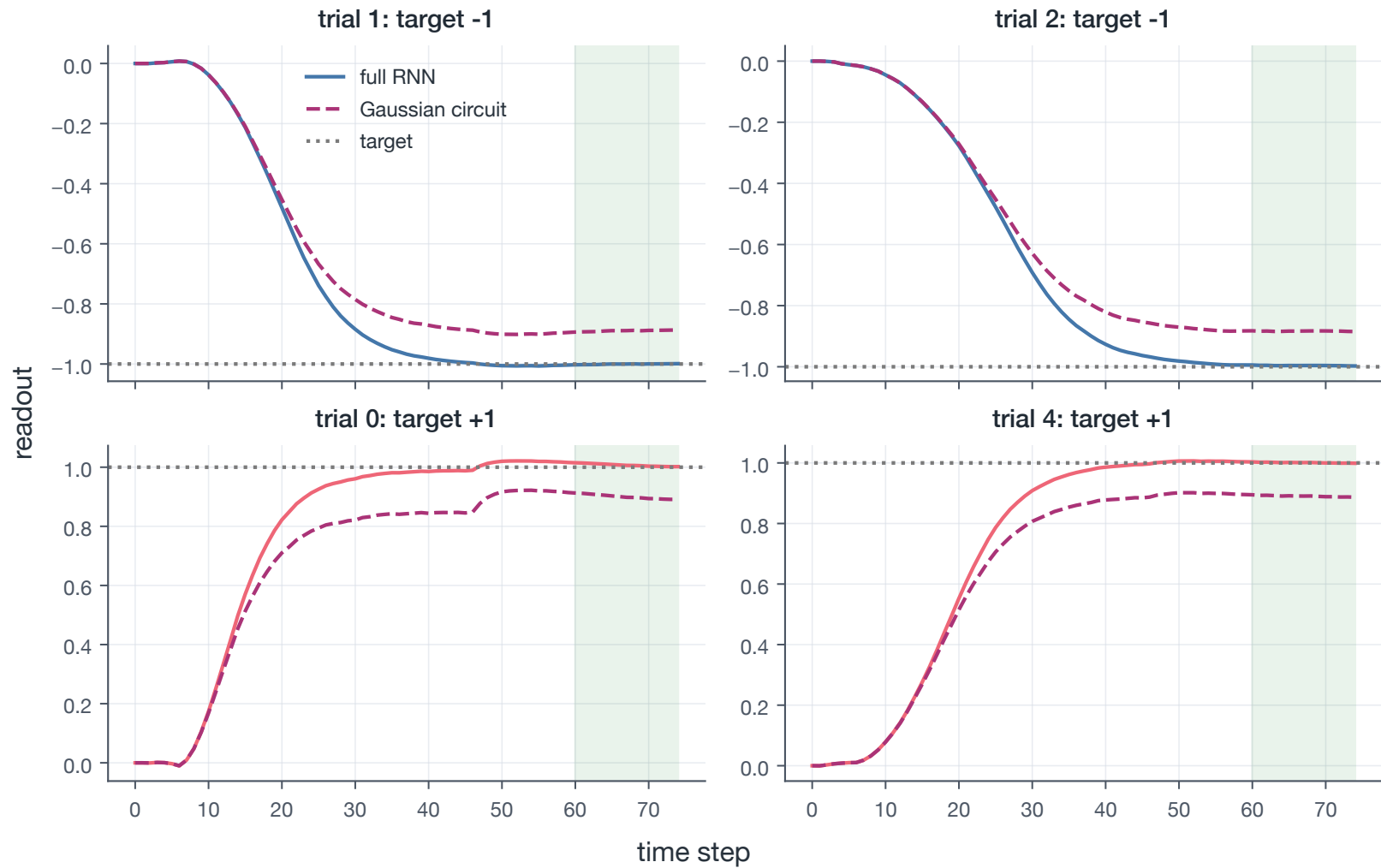
Full rank-one RNN and its Gaussian circuit
