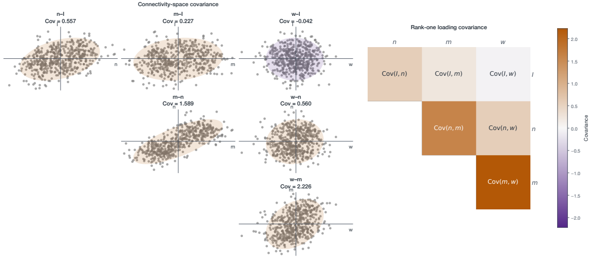
Figure 7. Pairwise loading-space point clouds and the covariance heatmap for the current N = 512 rank-one run. The three task-relevant population covariances are approximately (\sigma_{nl}, \sigma_{mn}, \sigma_{mw}) = (0.556, 1.586, 2.222) .
