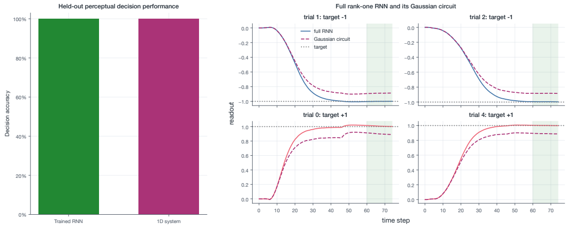
Figure 11. Accuracy between trained RNN and ID system (left), and representative trajectories (right).
