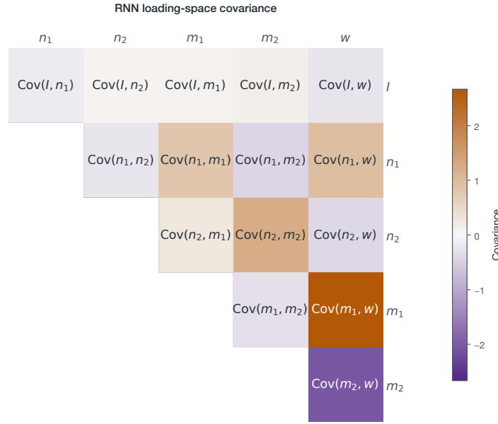
Figure 17. Upper-triangular covariance matrix of the six-dimensional loading space (l, n_1, n_2, m_1, m_2, w) . Positive within-mode covariances slow the latent dynamics, while opposite-signed cross-mode covariances generate the observed oscillatory dynamics.
