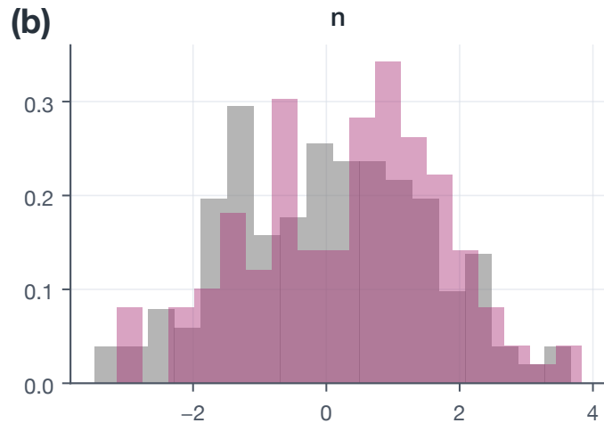
Empirical vs Gaussian samples
