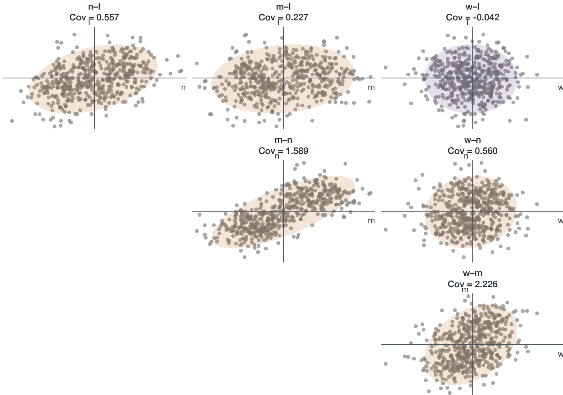
Connectivity-space covariance
