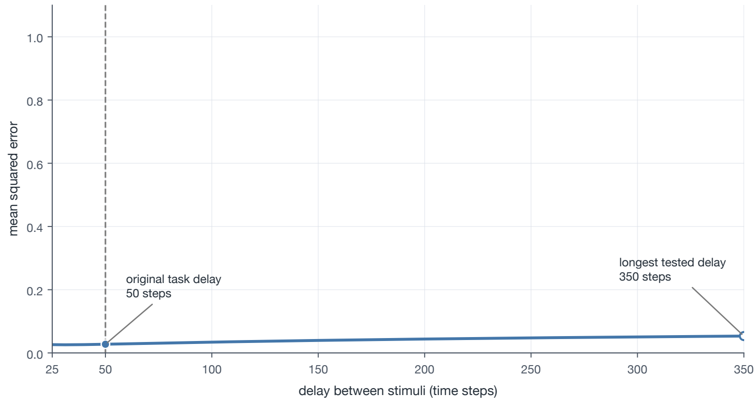
Paper-covariance prediction error over extended delays
