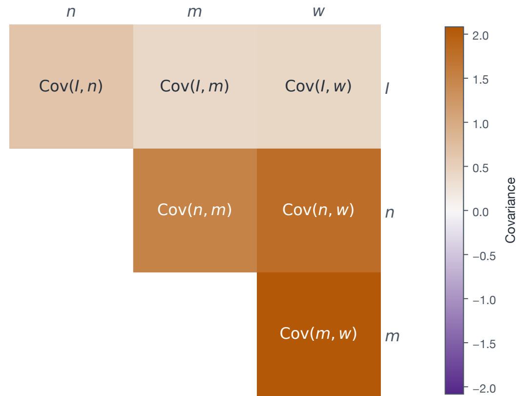
Gaussian-sample covariance
