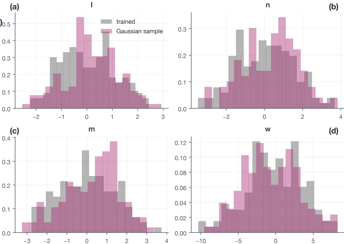
Empirical vs Gaussian samples
