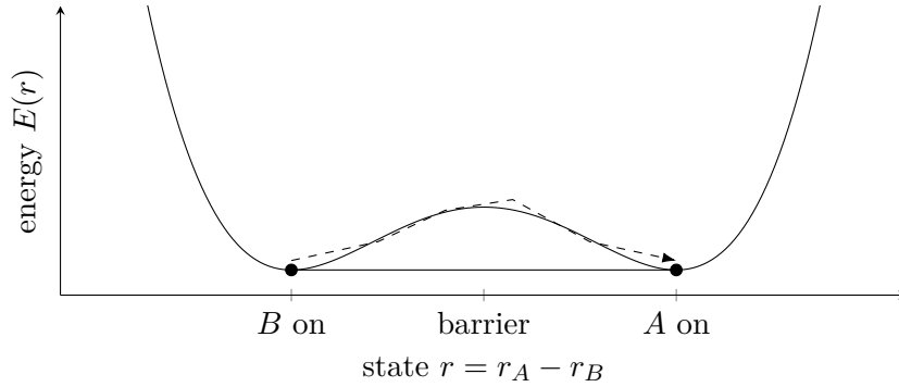
Figure 15: Attractor picture for noise-driven switching. The system usually sits near one energy minimum. A large enough fluctuation can move it over the barrier into the other basin. Adaptation lowers the effective barrier for the currently dominant percept.
