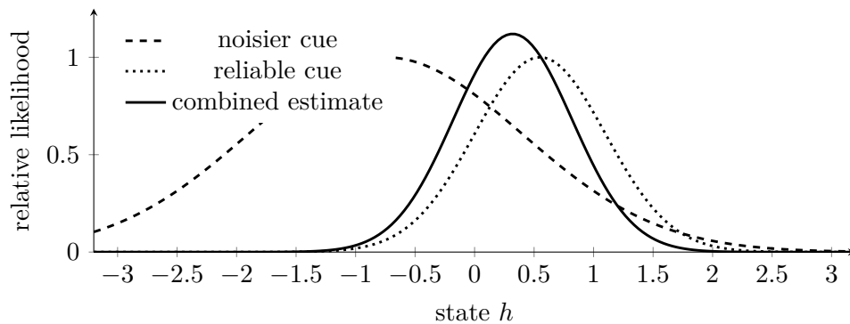
Figure 17: Gaussian cue combination. The combined estimate lies closer to the more reliable cue and has lower variance than either cue alone.
