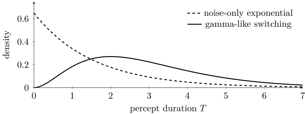
Figure 14: Percept-duration distributions help distinguish mechanisms. A fixed-barrier noise model gives memoryless exponential escape times. Adaptation plus noise naturally produces a more peaked, gamma-like distribution because the escape probability changes with time since the last switch.
