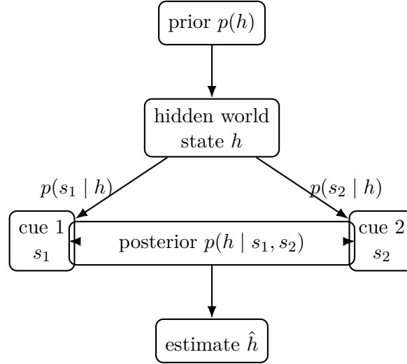
Figure 16: Generative model for cue integration. The world state causes sensory measurements, and inference runs in the opposite direction: combine the cues to estimate the hidden state.
