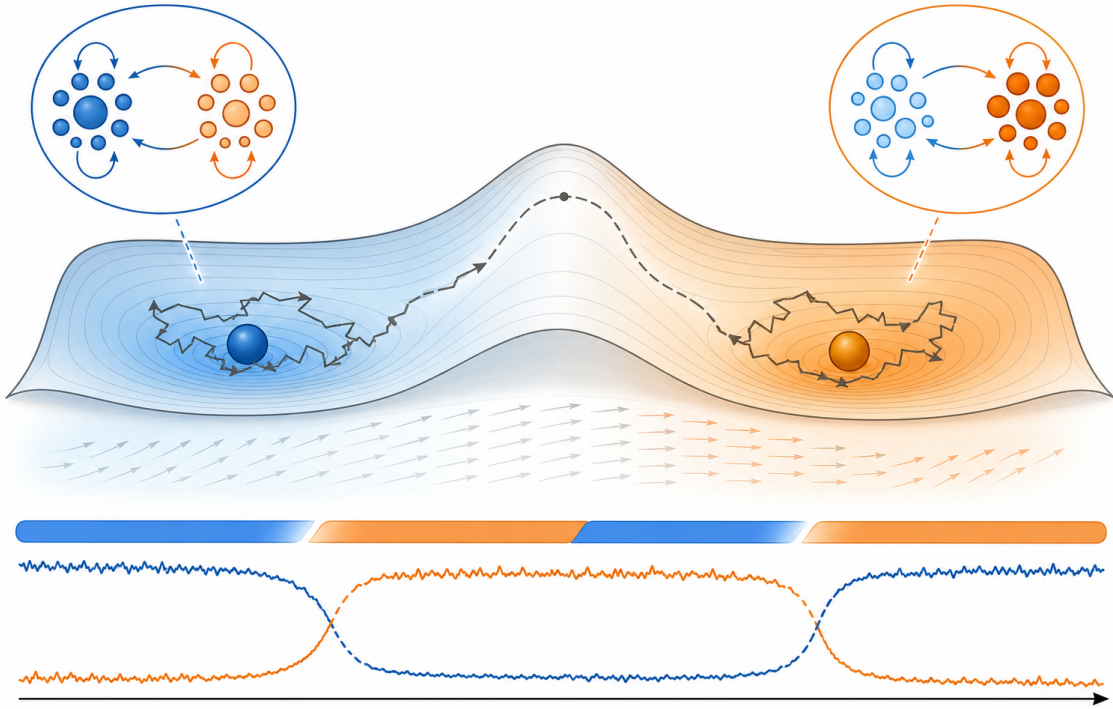
Figure 12: Bistable perception can be pictured as motion between two attractor basins. Competition makes one percept dominate at a time; slow adaptation reshapes the currently occupied basin; noise can then push the state across the barrier into the other interpretation.
