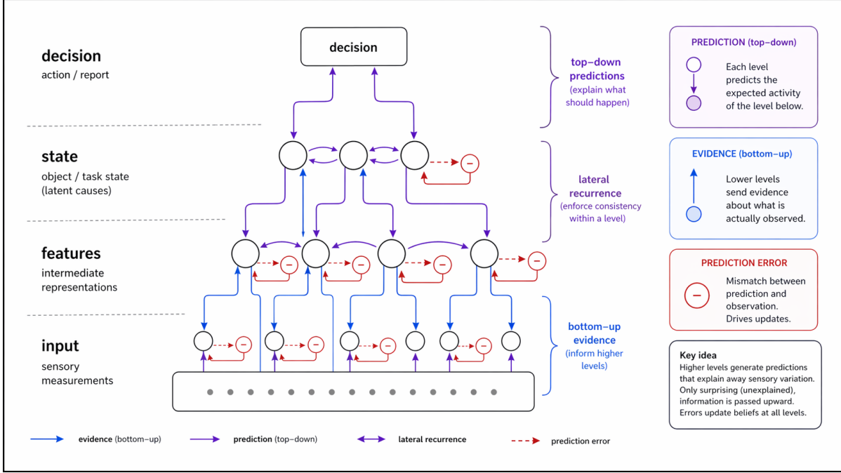
Figure 18: A compact view of hierarchical inference. Bottom-up evidence constrains higher latent states, top-down predictions explain expected sensory structure, lateral recurrence enforces consistency within a level, and prediction errors update the representation.
