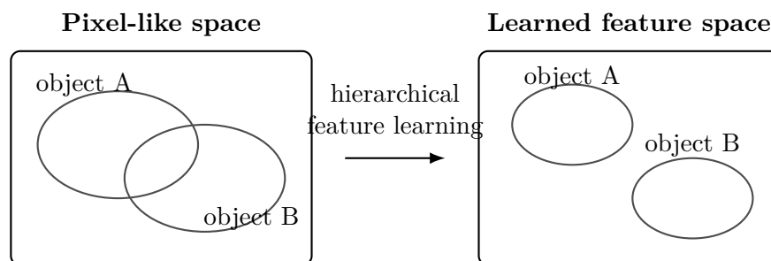
Figure 4: The geometric picture emphasized in the lecture. In raw image coordinates, object manifolds are tangled together. A good representation transforms them into a space where object identity is easier to separate.
