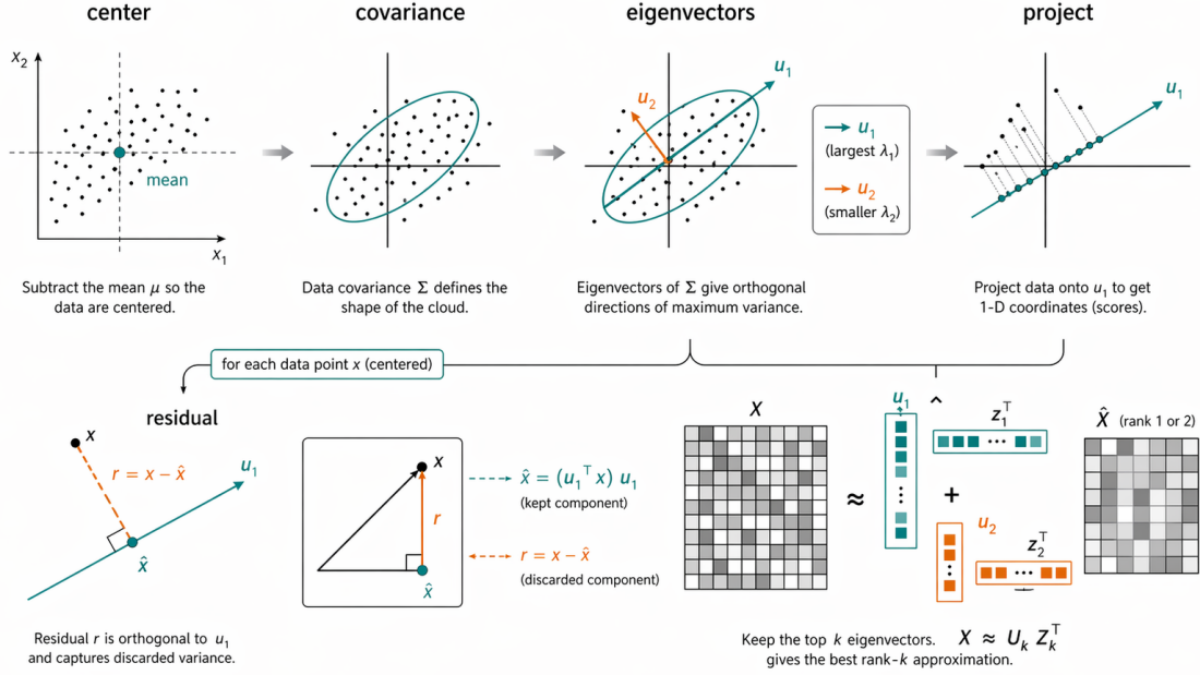
Figure 6: PCA as spectral compression. Centering removes the mean, the covariance ellipse reveals directions of variation, eigenvectors provide orthogonal coordinates, projection keeps high-variance coordinates, and residuals are the discarded orthogonal variation.
