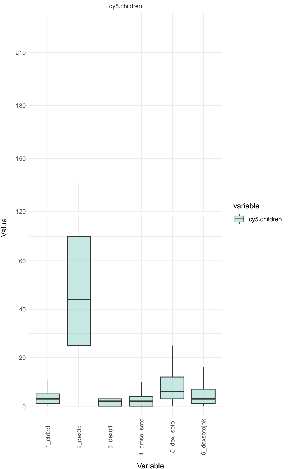
Box Plot Comparison of cy3, a594, cy5, cy7 Across Files
