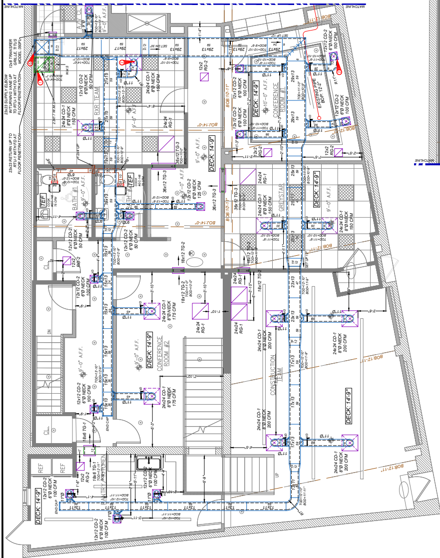
HVAC FIRST FLOOR SHOP DRAWING (1 OF 2) SCALE: 3/8" = 1'-0"
