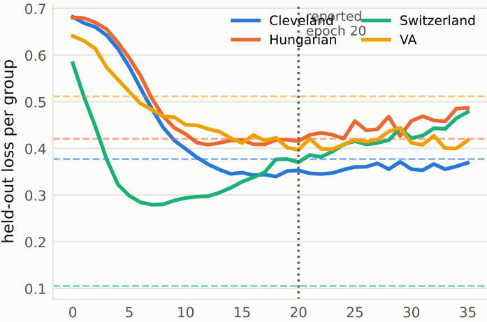
Fed-Heart · \gamma 0.02, per-epoch (paper's \lambda setting)
