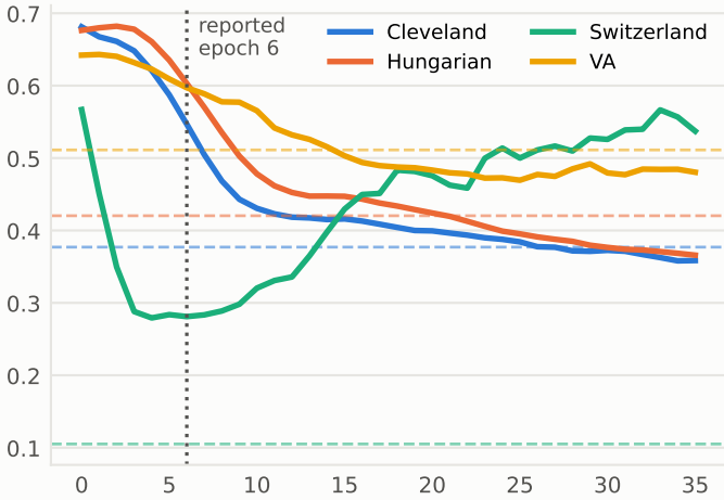
Fed-Heart · \gamma 0.5, per-step
