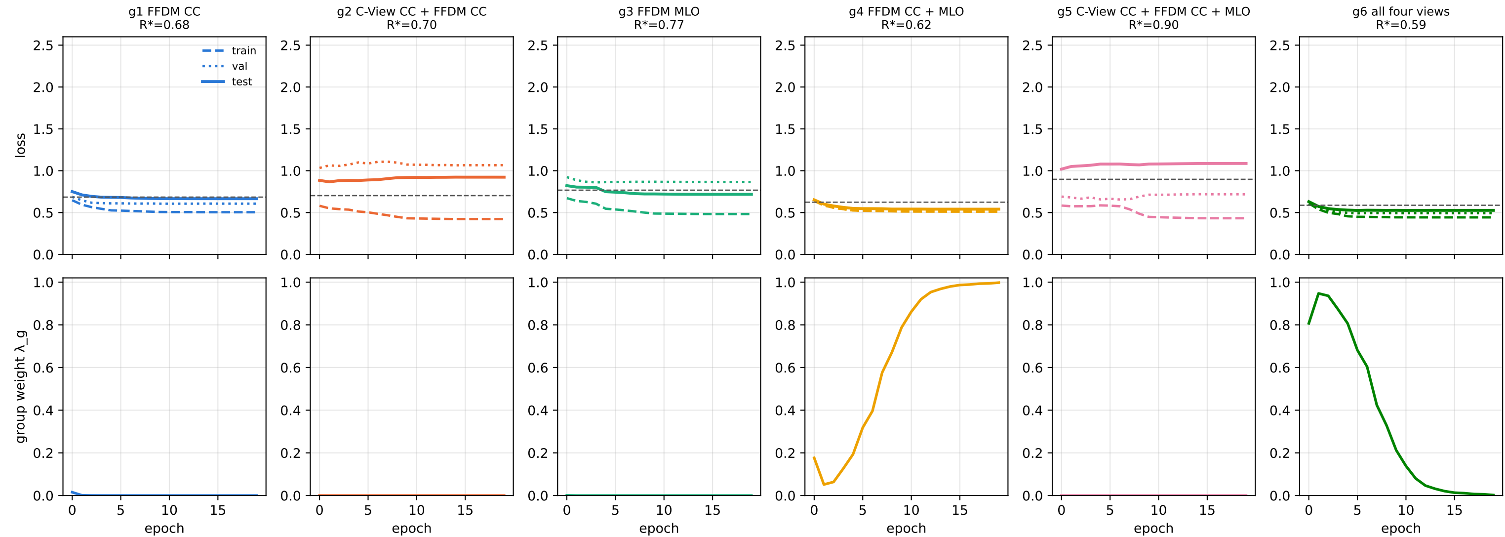
EMBED — ours: anchors + Regret-DRO: per-group loss (train dashed, val dotted, test solid) and group weight, seed 0 (uniform init, \gamma 2.0, train-signal schedule)
