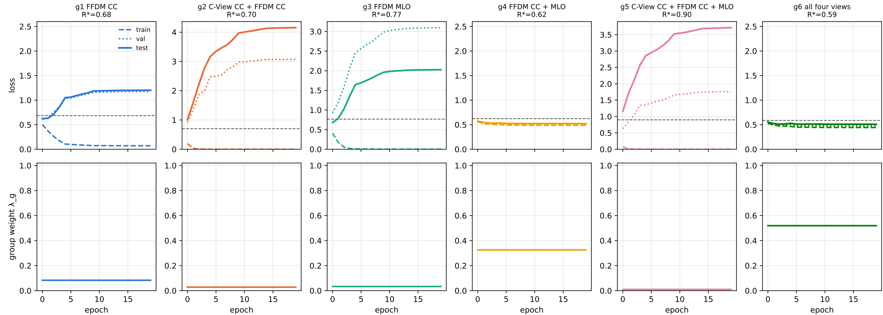
EMBED — Regret-DRO: per-group loss (train dashed, val dotted, test solid) and group weight, seed 0 (uniform init, \gamma 2.0, train-signal schedule)
