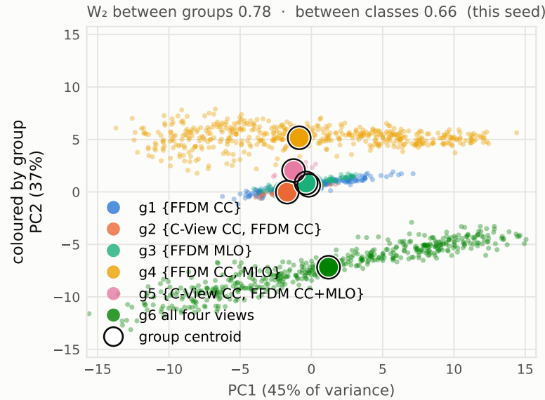
No anchors: per-group encoders + Regret-DRO
