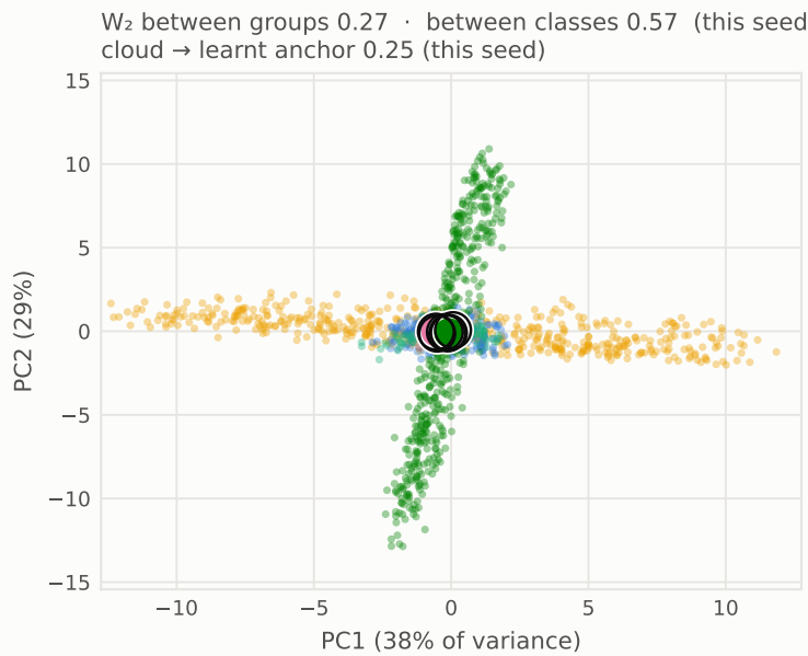
Class anchors: per-group encoders + anchors + Regret-DRO (ours)
