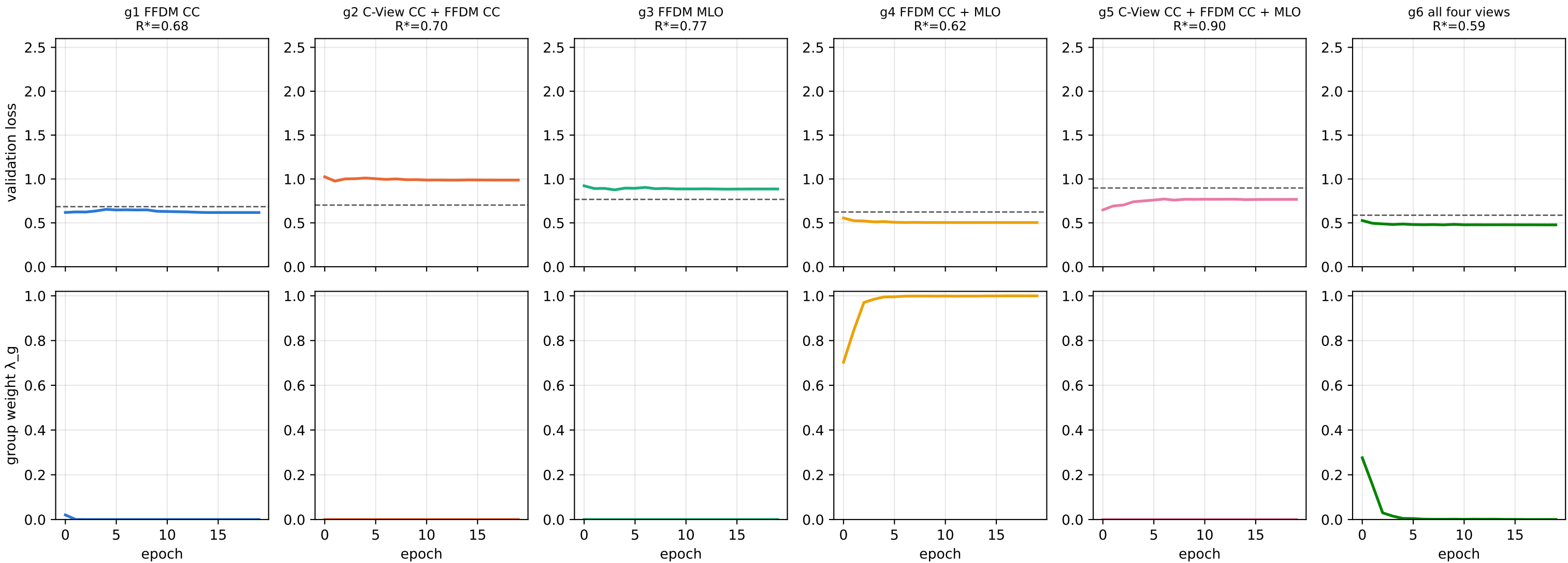
EMBED — GroupDRO: per-group validation loss and group weight, seed 0 (uniform init, \gamma 2.0, train-signal schedule)
