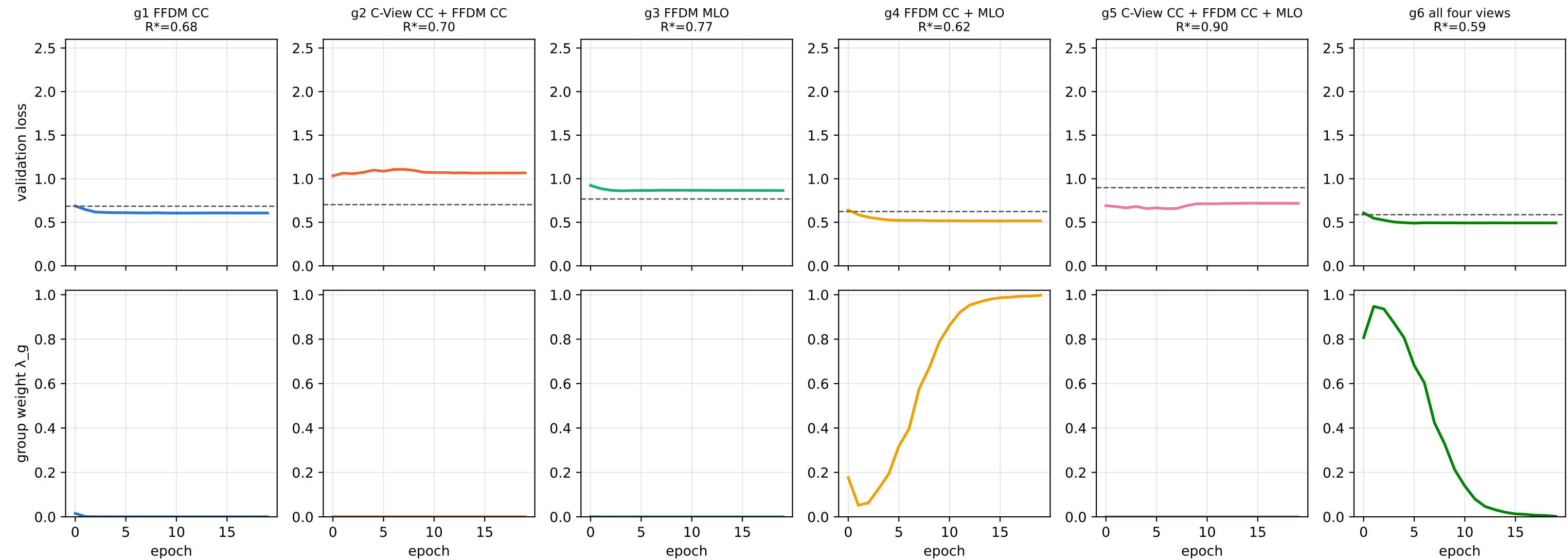
EMBED — ours: anchors + Regret-DRO: per-group validation loss and group weight, seed 0 (uniform init, \gamma 2.0, train-signal schedule)
