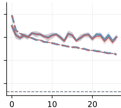
+ labs R^*=0.26
