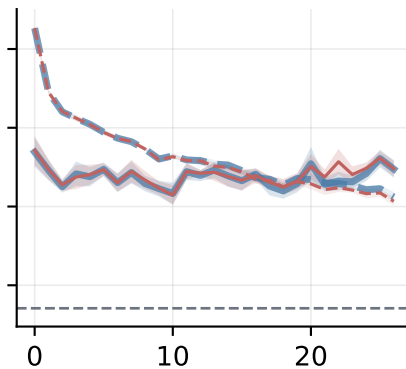
+ exam R^*=0.27
