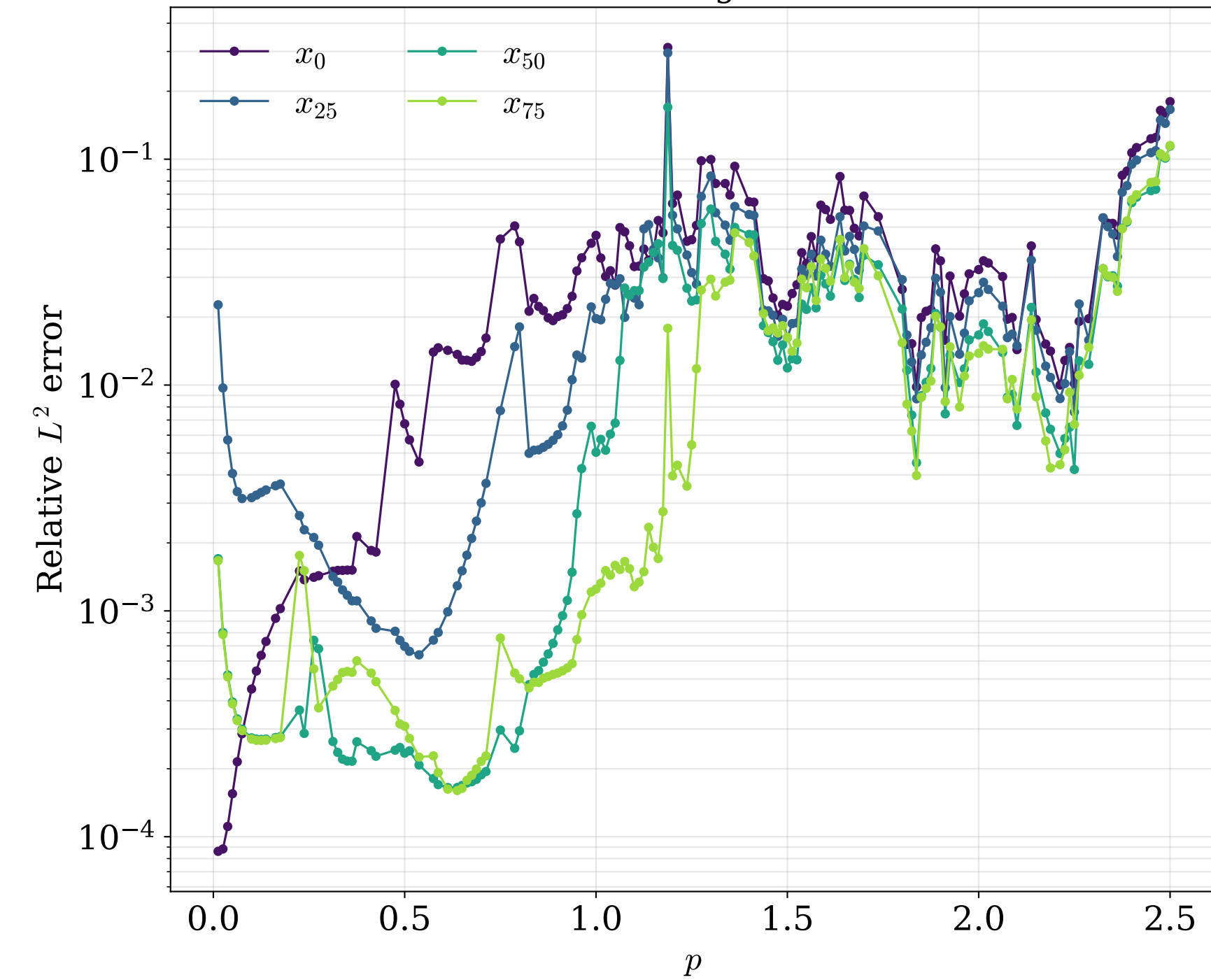
Training set
