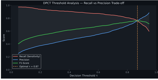
Fig. 3 Threshold optimisation curve (F1-score, Precision, Recall vs. \tau ) on the held-out test set. The globally optimal point is \tau^* = 0.87 (Recall = 0.759, Precision = 0.762). The deployed model uses the fold-specific threshold \tau = 0.88 .
