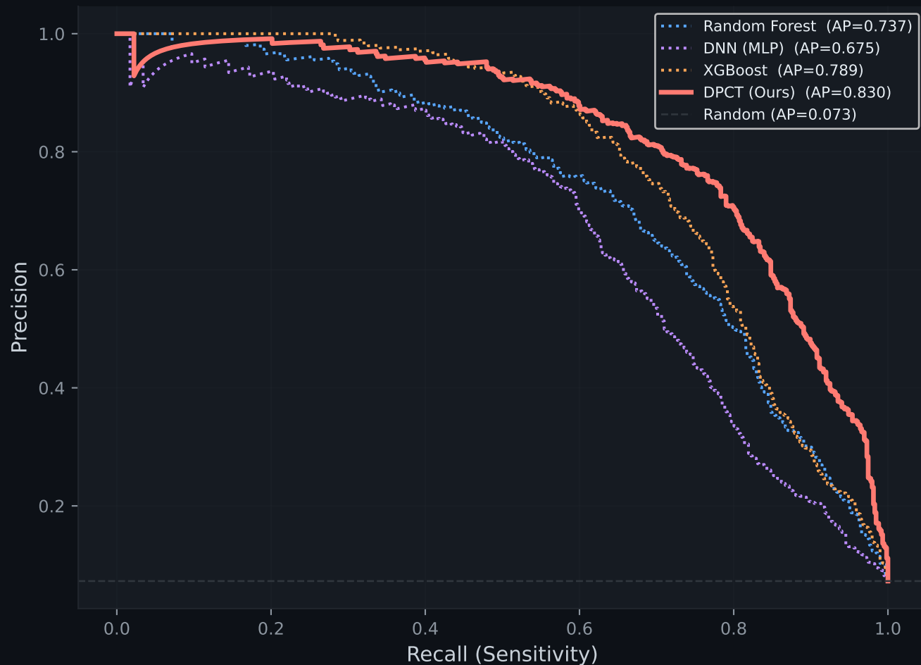
Precision-Recall Curves
