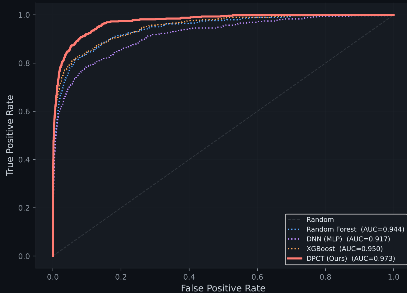
ROC Curves
