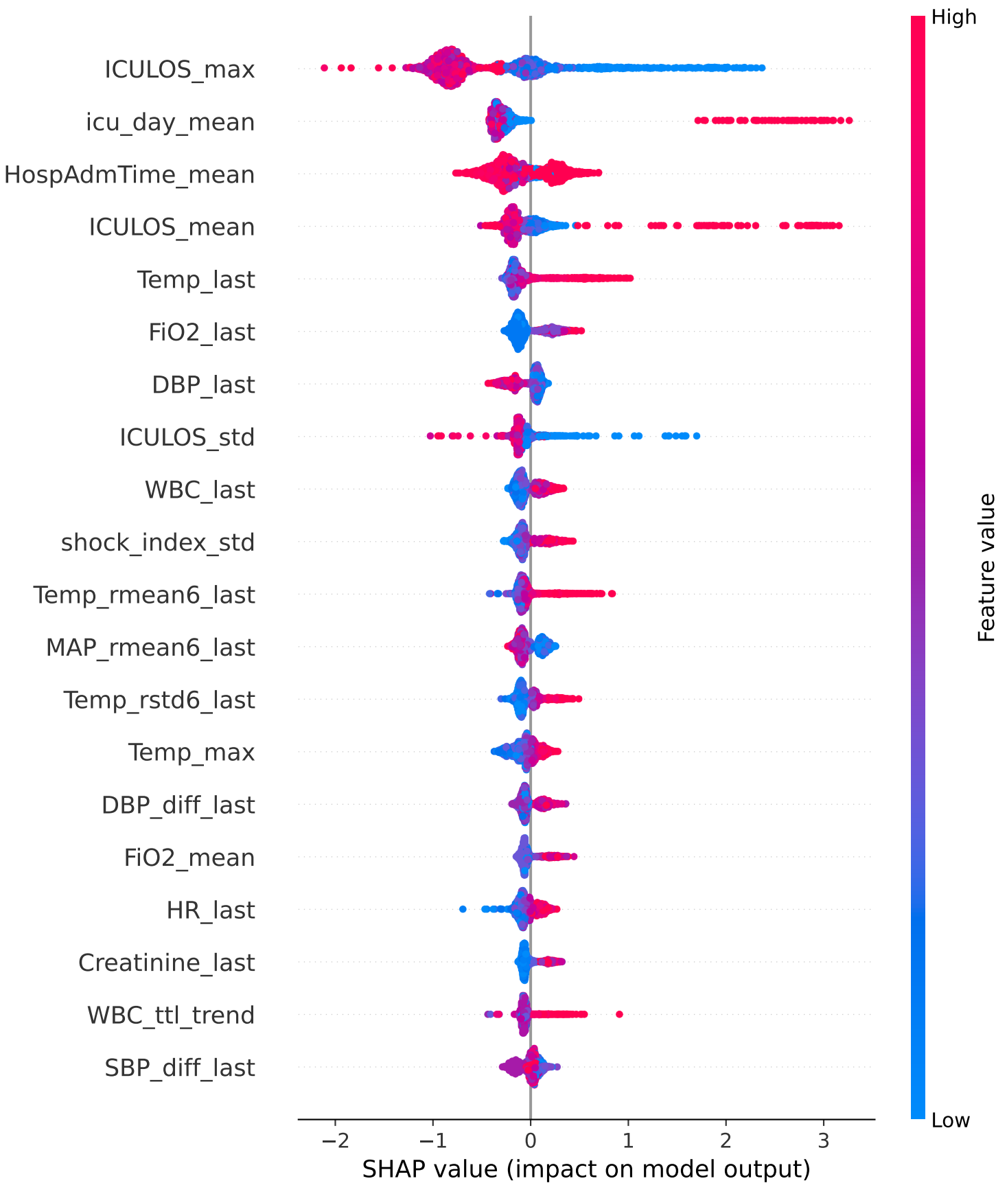
SHAP Feature Importance (XGBoost) — Top 20 Features
