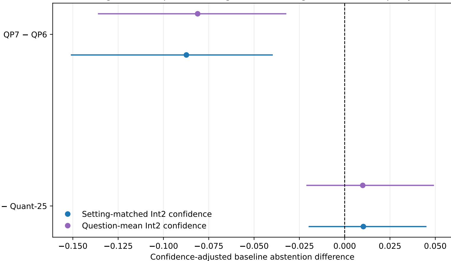
Original consequence-setting contrasts using Int2 confidence proxy
