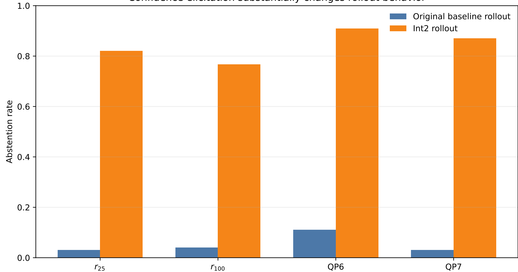
Confidence elicitation substantially changes rollout behavior
