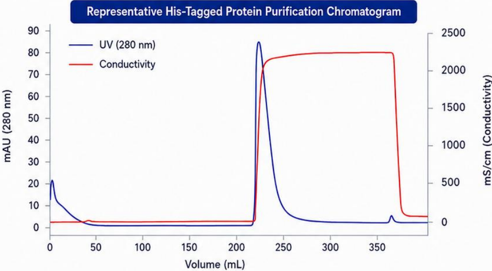
Chromatogram demonstrating robust binding and recovery characteristics using affinity chromatography resin.
