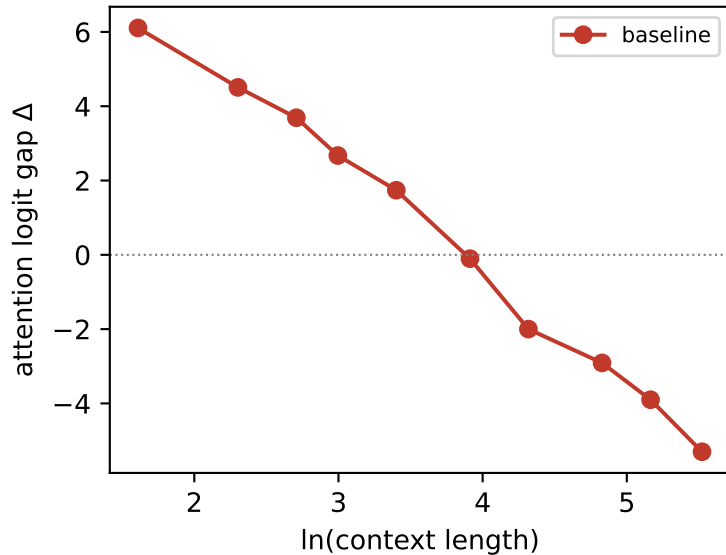
Gap vs length (argmax, nope)
