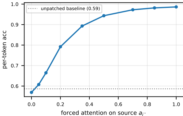
Selection drives accuracy ( r=+0.89 )
