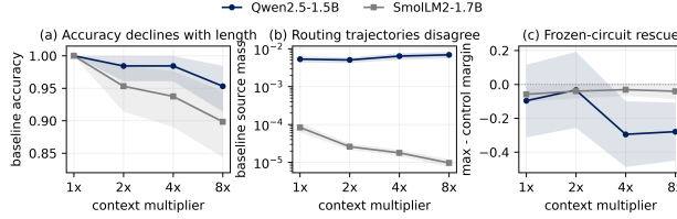
Figure 5: Matched natural-QA length ladder (seed 0; the four-passage circuit is frozen once per seed and reused at every length, and the additional Qwen seed is in the supplementary material). Bands are paired bootstrap 95% intervals over n = 128 examples per cell. From 4 to 32 passages, accuracy falls (a), source routing moves in opposite directions across models (b), and frozen-circuit rescue stays flat or weakens (c).
