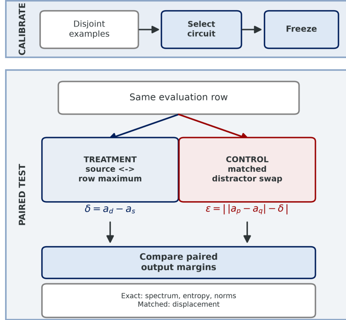
Figure 1: Paired causal protocol. A circuit selected on disjoint calibration data is frozen before treatment and control are applied to the same evaluation row. Both paths preserve the spectrum; the natural QA control additionally minimizes displacement mismatch in Equation 6.
