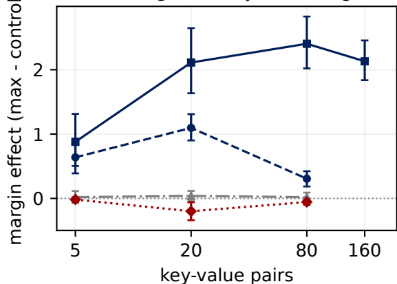
(a) Routing varies by model regime
