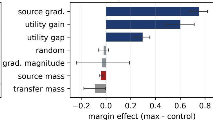
(b) Output-aware selection
