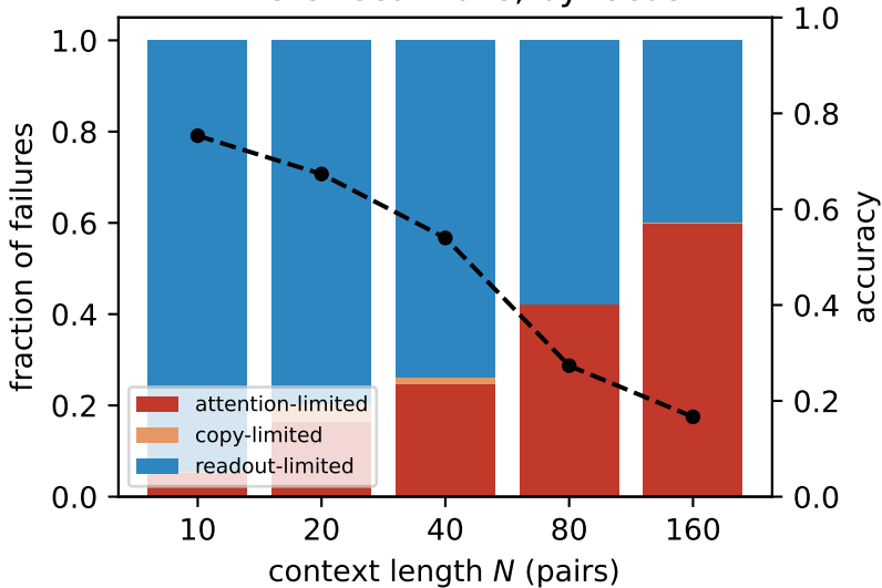
Where recall fails, by locus
