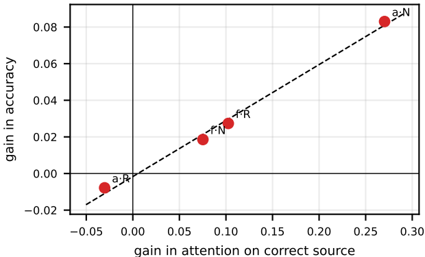
Accuracy gain tracks attention gain ( r=+1.00 )
