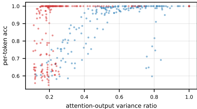
accuracy vs variance ( r=0.45 )
