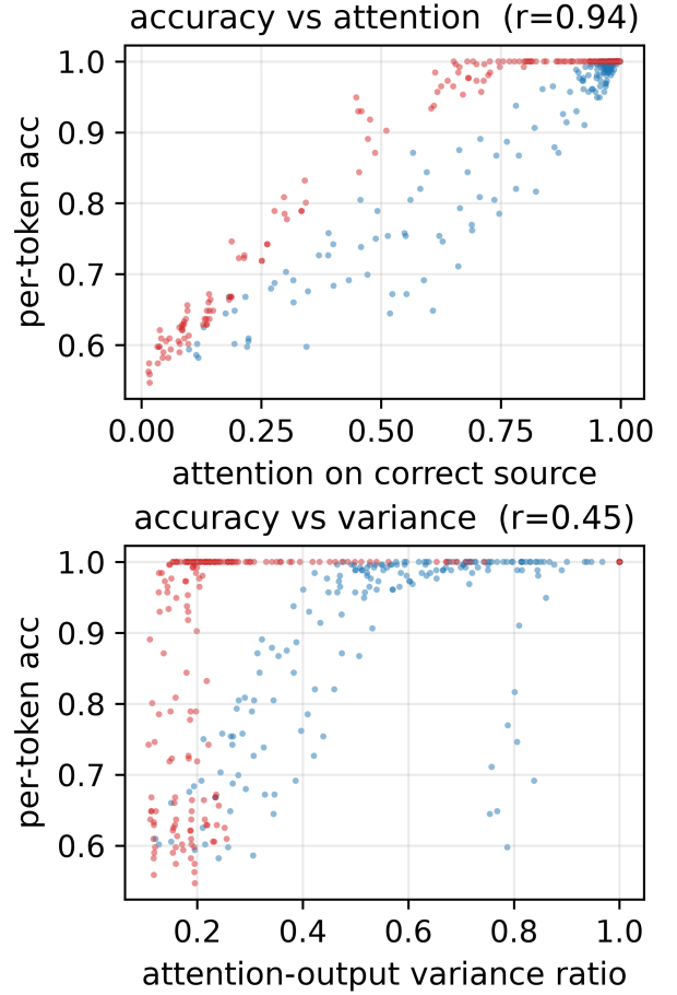
Figure S1: Controlled baselines pooled over lengths and seeds. Accuracy is tightly related to attention on the task-required source (top), but only diffusely related to attention-output variance (bottom).
