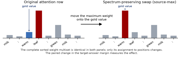
Figure 1: A fixed-spectrum swap (FSS) on in-context key-value recall, one of the conditions we run. Both rows hold the same sorted weights; source-max moves the maximum onto the gold value (“warm”) while preserving the spectrum, and the paired target-margin change measures the effect. The matched control instead swaps two task-irrelevant weights, so treatment and control share spectrum and displacement.
