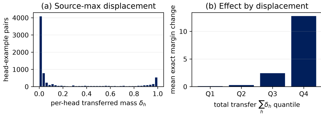
Figure S7: Controlled source-max displacement. Left: the per-head transferred-mass distribution. Right: exact margin change increases with total circuit transfer. Individual swaps are vacuous for 18.5% of head-example pairs, while 8.4% of complete eight-head circuits are entirely vacuous.
