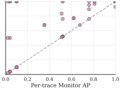
Qwen-3.5
