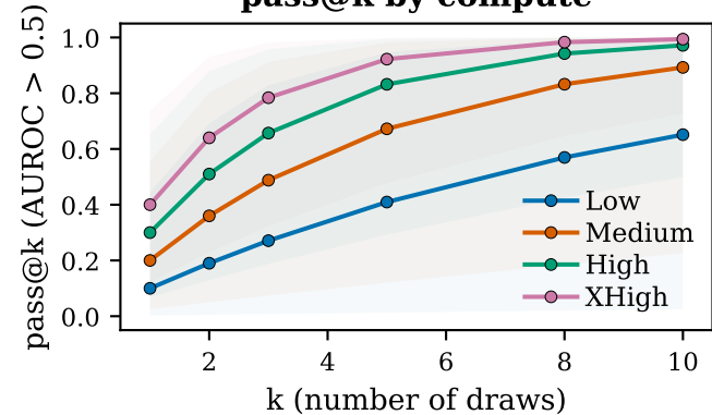
pass@k by compute
