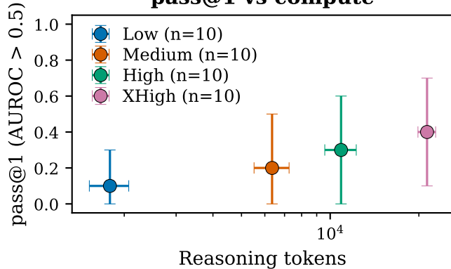
pass@1 vs compute
