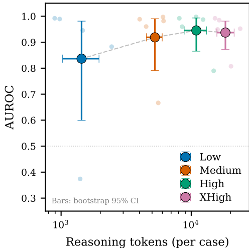
(a) Absolute AUROC
