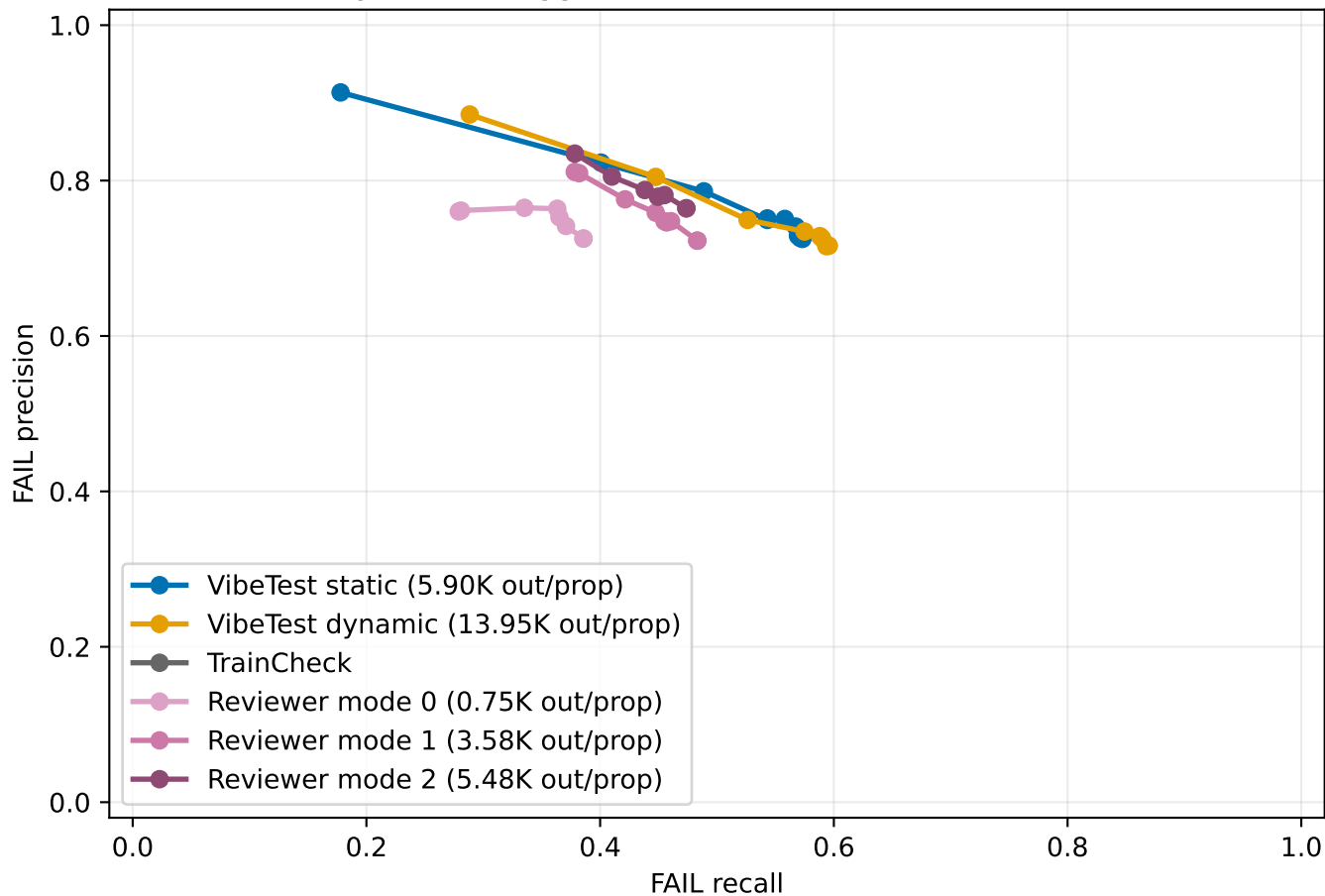
Synthetic Kaggle Qwen3.6: FAIL Precision-Recall
