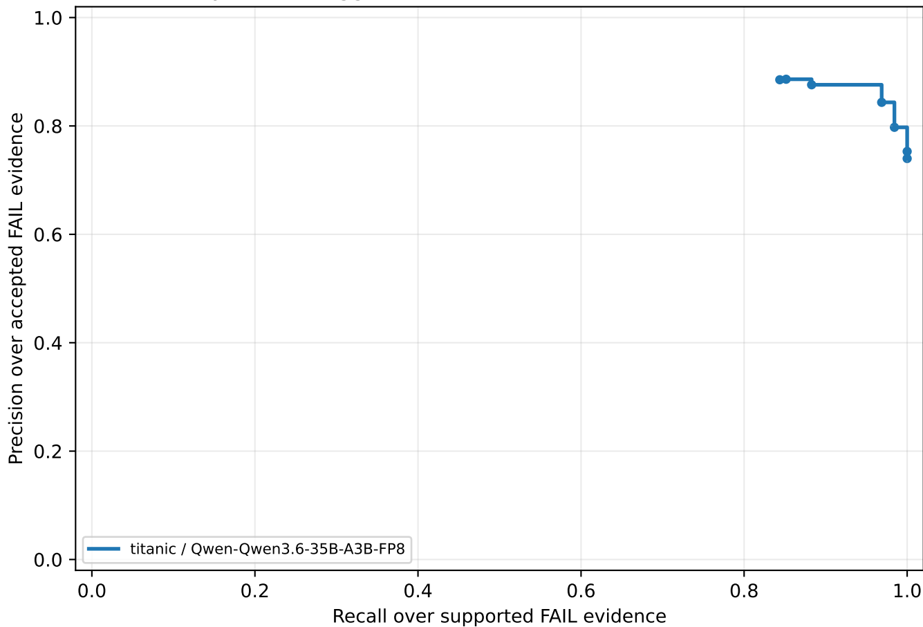
Synthetic Kaggle Qwen3.6 Titanic Evidence Verifier PR
