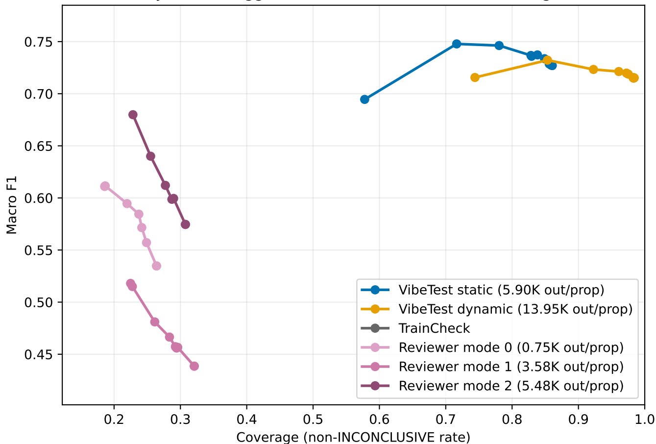
Synthetic Kaggle Qwen3.6: Selective F1 vs Coverage
