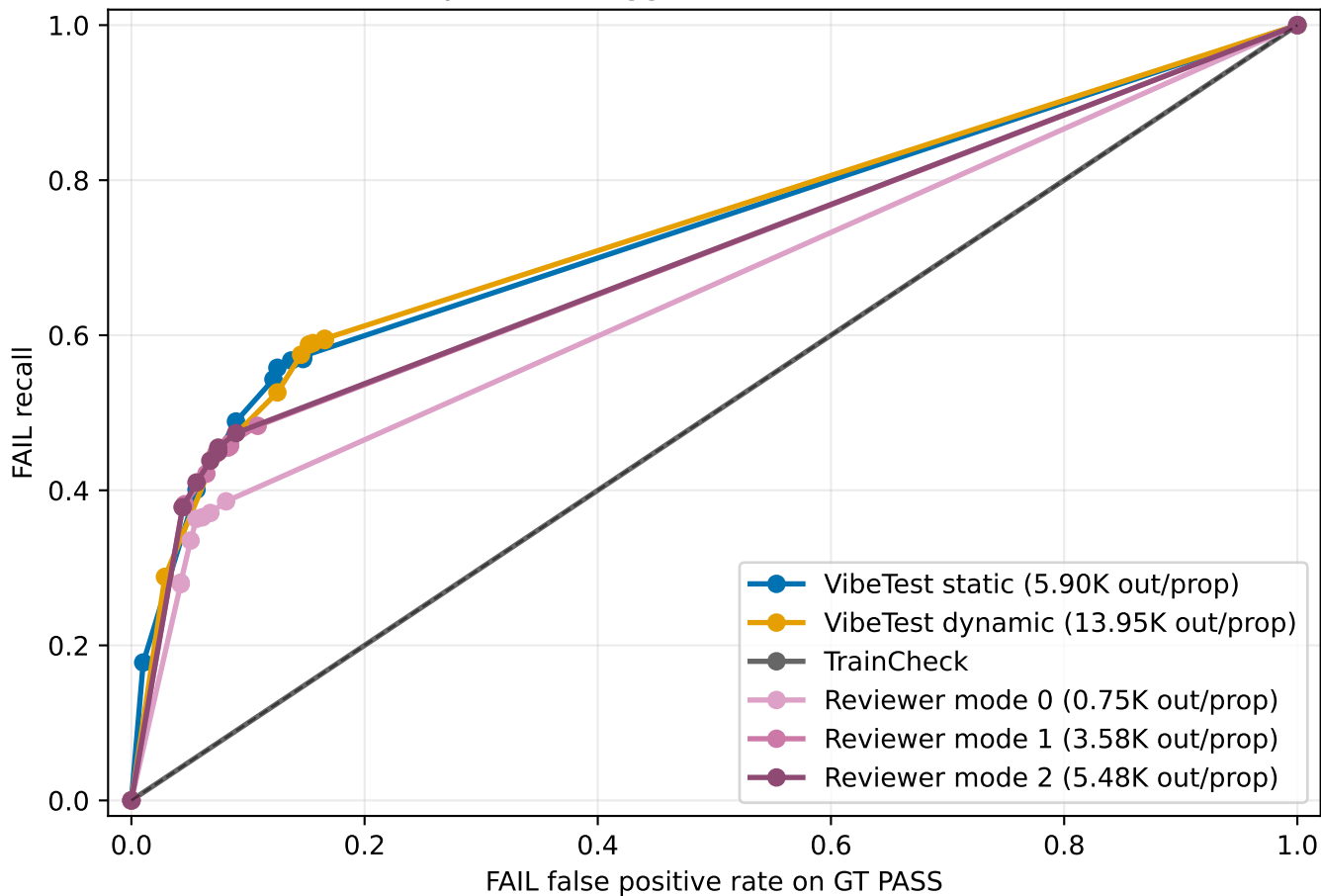
Synthetic Kaggle Qwen3.6: FAIL ROC
