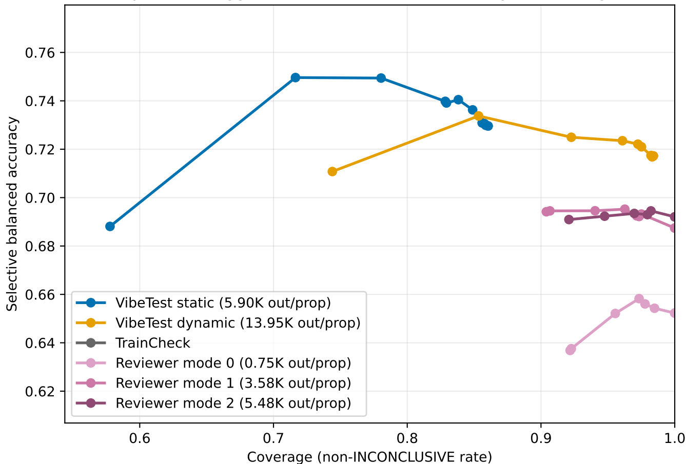
Synthetic Kaggle Qwen3.6: Selective Reliability vs Coverage
