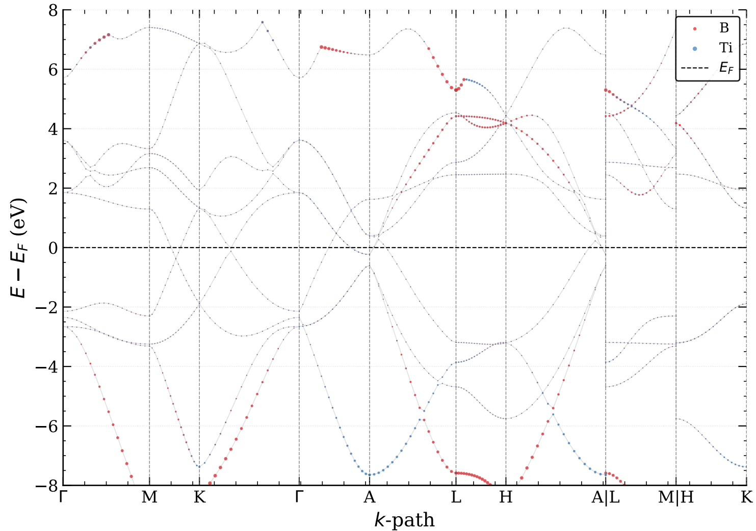
(a) Band Structure
