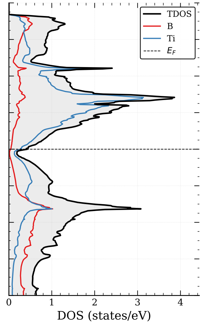
(b) Density of States
