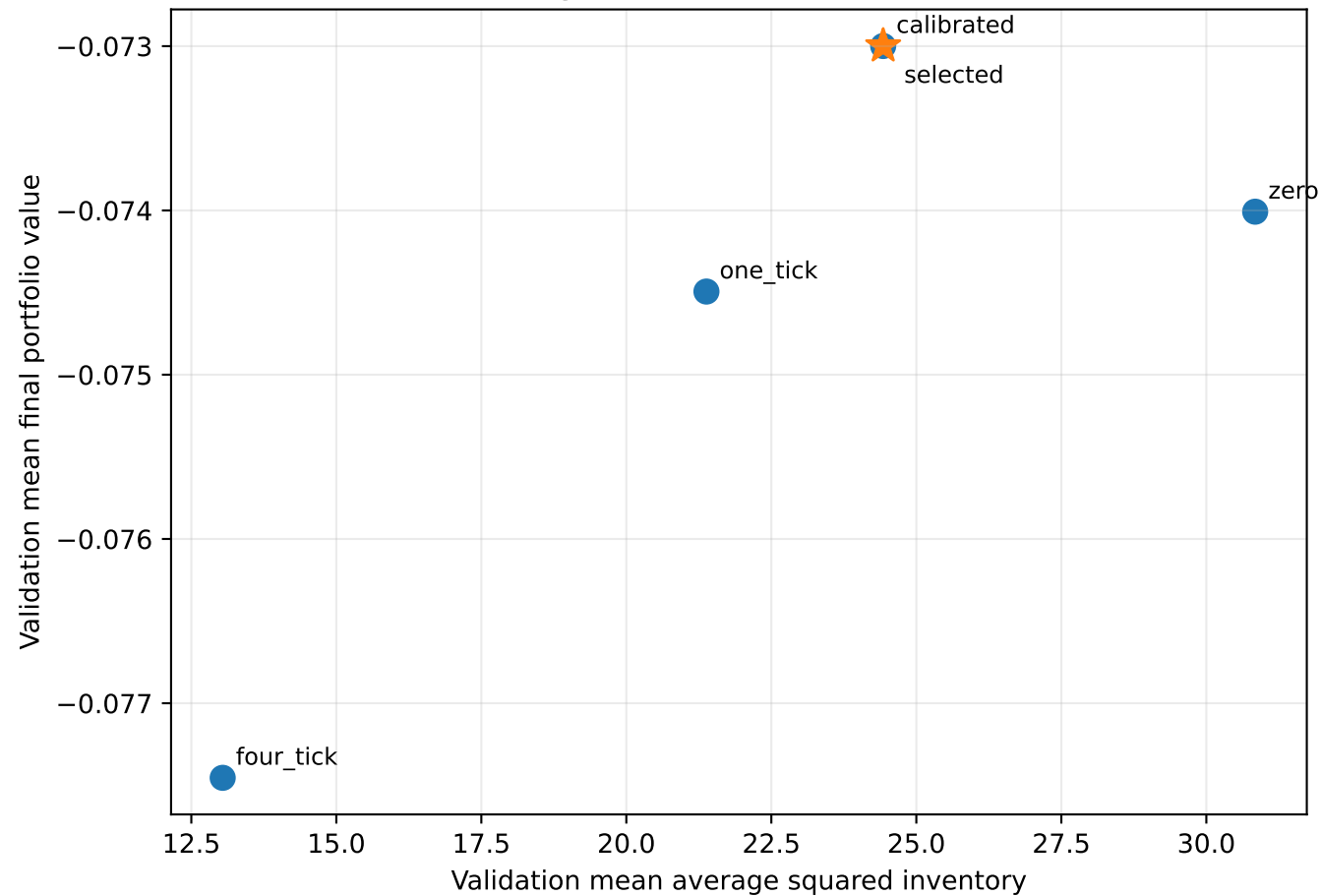
AS validation gamma selection: risk-return frontier
