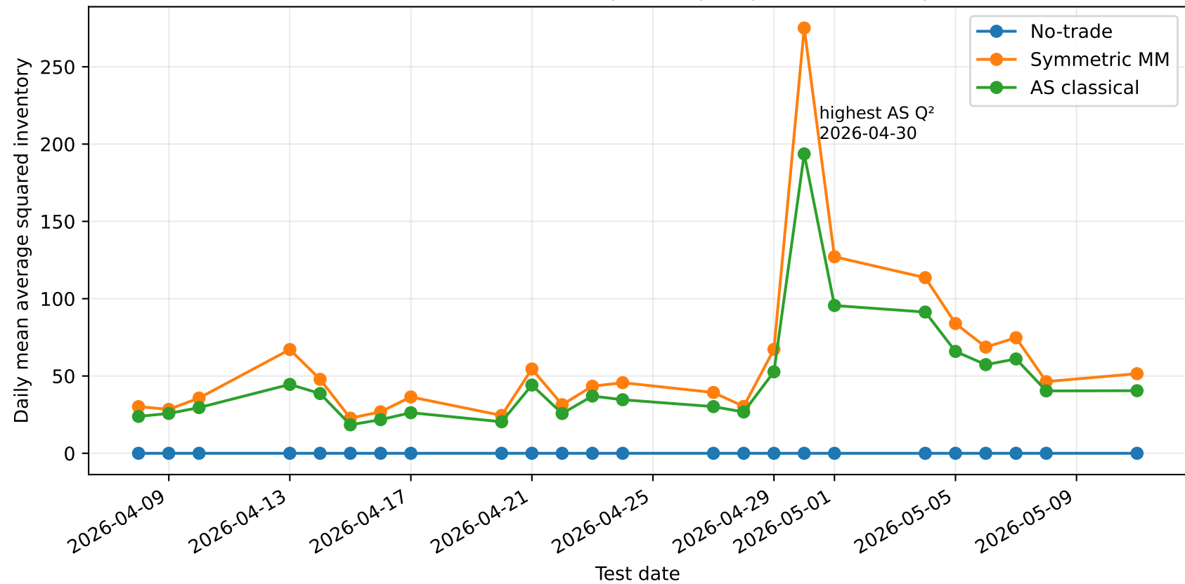
AS test benchmark: daily average squared inventory
