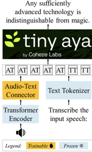
Figure 1: LisTaya
