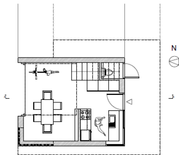
PLAN 1
